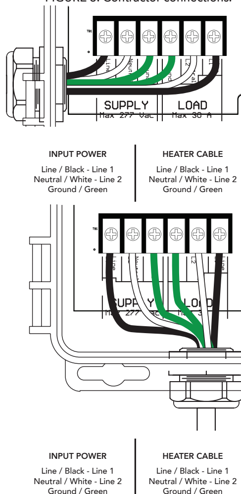
FIGURE 3. Contractor connections.
