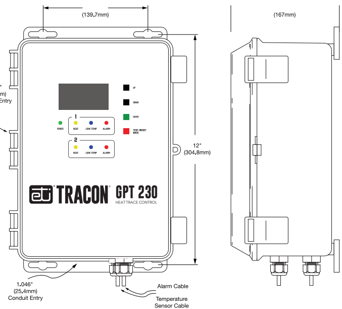
FIGURE 2. Mounting dimensions.
