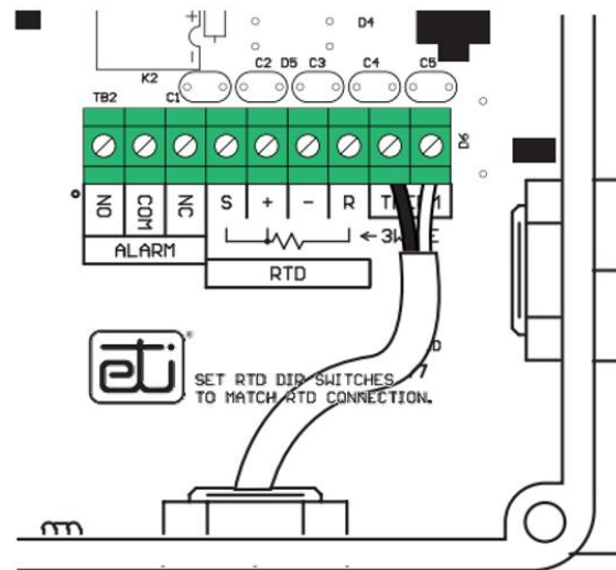
FIGURE 4. Temperature sensor wiring
