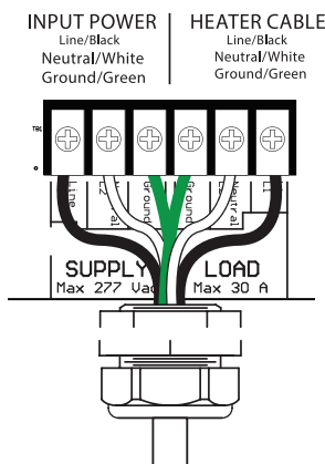
FIGURE 3. Contractor connections.
