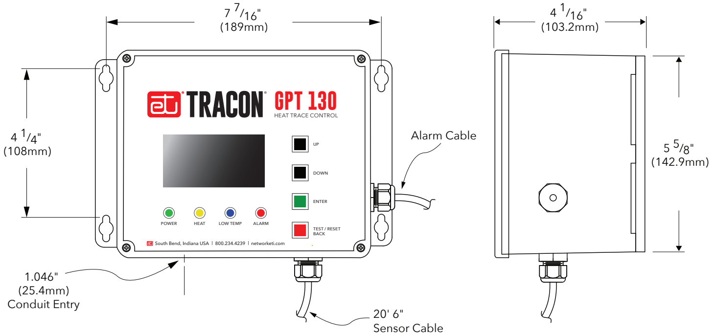
FIGURE 2. Mounting dimensions.
