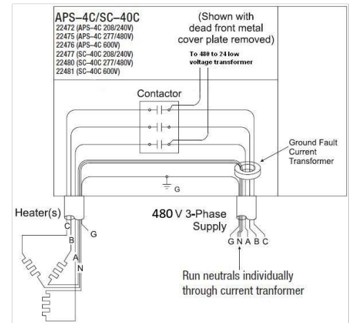
FIGURE 15. APS-4C and SC-40C Three Phase Y Connection(WYE).
