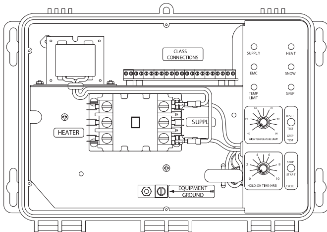
FIGURE 15. APS-4C and SC-40C Three Phase Y Connection(WYE).
