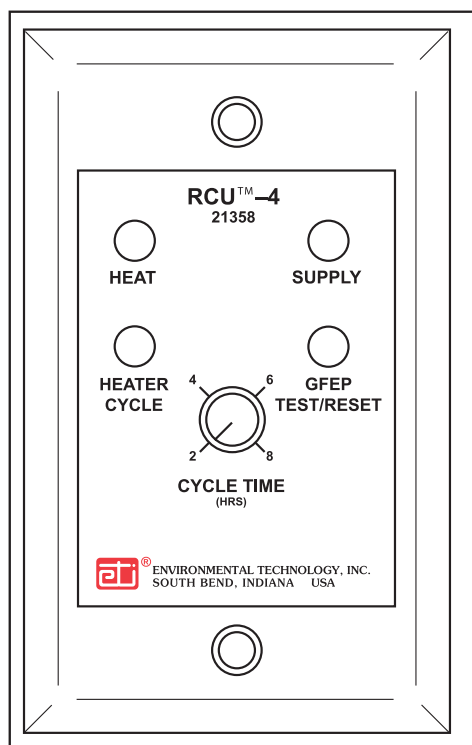
FIGURE 5. RCU-3 (above), RCU-4
