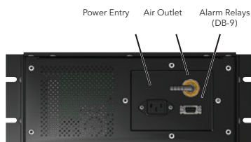
FIGURE 2. EDH-4 Components
