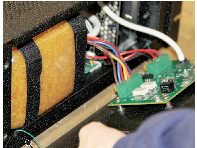
FIGURE 10. Desiccant Bottle Removal - Front Display Panel, clockwise from left: Open front panel; undo straps; disconnect tubing; ready; remove bottle; open or replace
