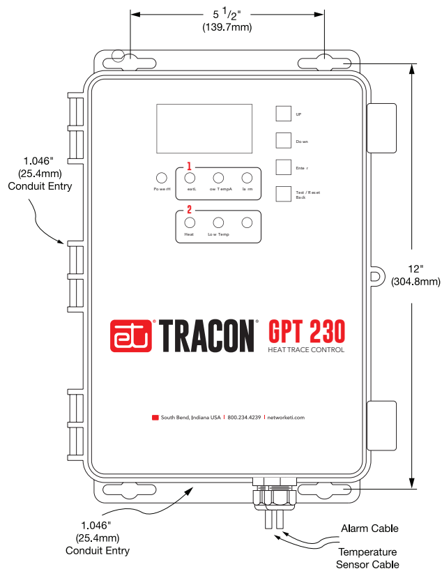
FIGURE 2. Mounting Dimensions
