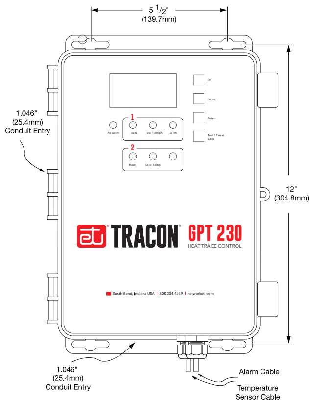
FIGURE 2. Mounting Dimensions
