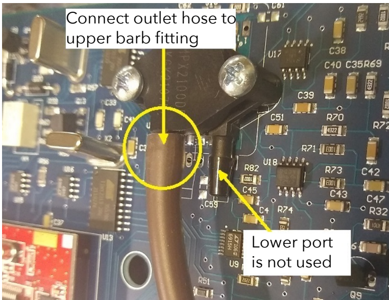
Figure 18 b. ALTERNATE PRESSURE TRANSDUCER UPPER PORT.
