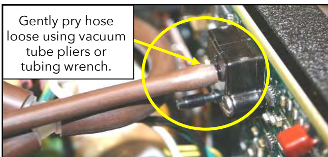
Figure 12. PRESSURE TRANSDUCER.
