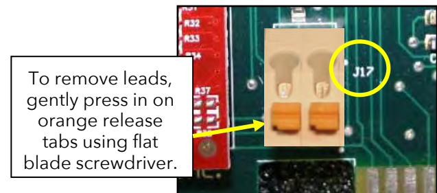
Figure 3. TERMINAL BLOCK J17.
