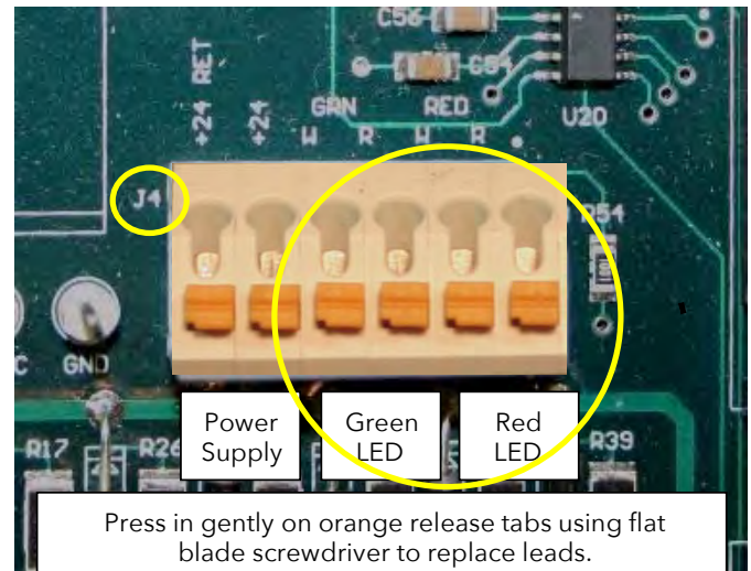
Figure 3. TERMINAL BLOCK J4.
