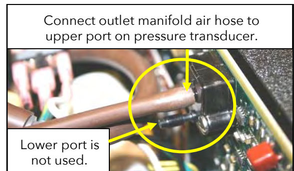
Figure 11. PRESSURE TRANSDUCER UPPER PORT.
